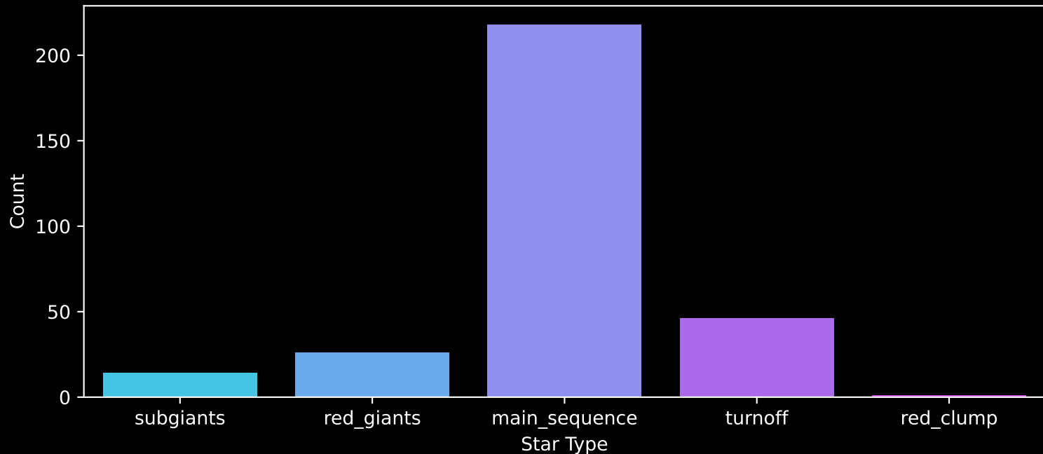
APOGEE DR17 Field: [sgr_tidal13] Count plot of Star Type
