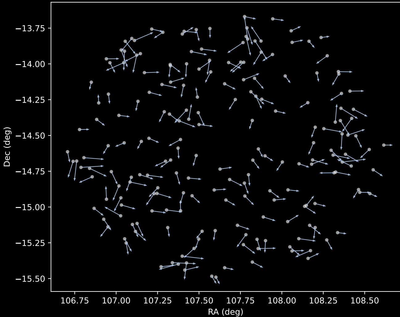
APOGEE DR17 Cluster 1 Proper Motion Vectors (n=198)
