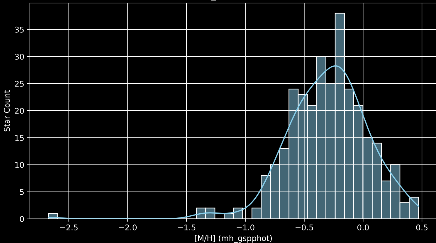
APOGEE DR17 Field: [sgr_tidal13 [M/H] (mh_gspphot) (n= 300)
