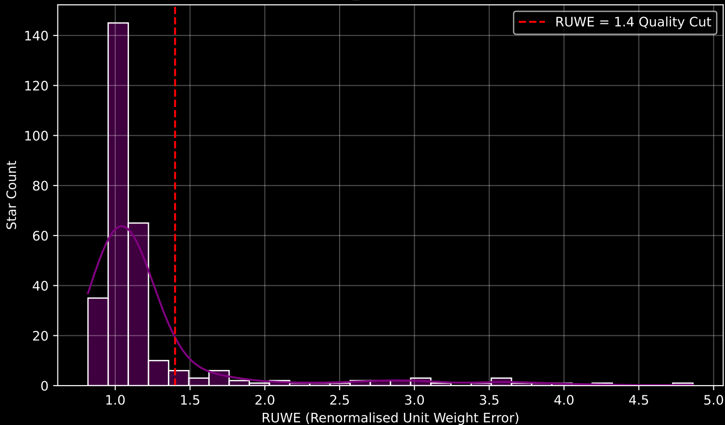
GAPOGEE DR17 Field [sgr_tidal13] RUWE Distribution (n= 297)
