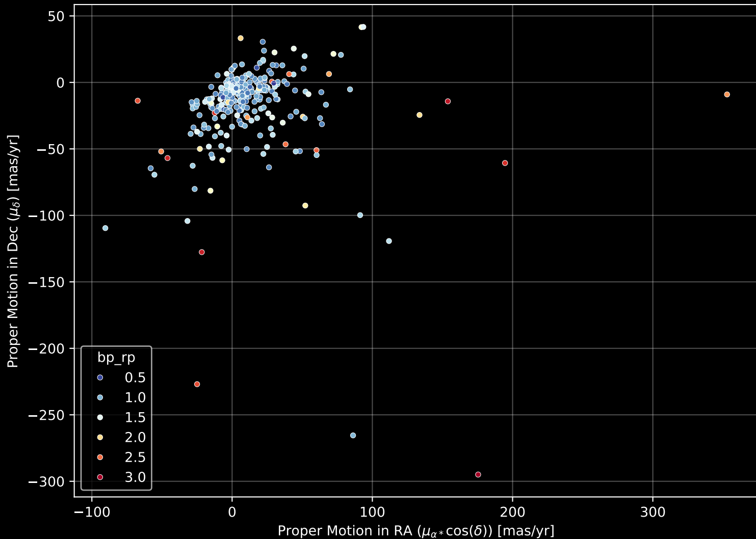
APOGEE DR17 Field: [sgr_tidal13] Proper Motion Diagram (n= 305)
