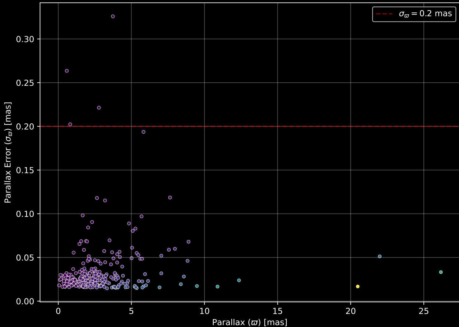
APOGEE DR17 Field: [sgr_tidal13] Parallax Quality (n= 305)
